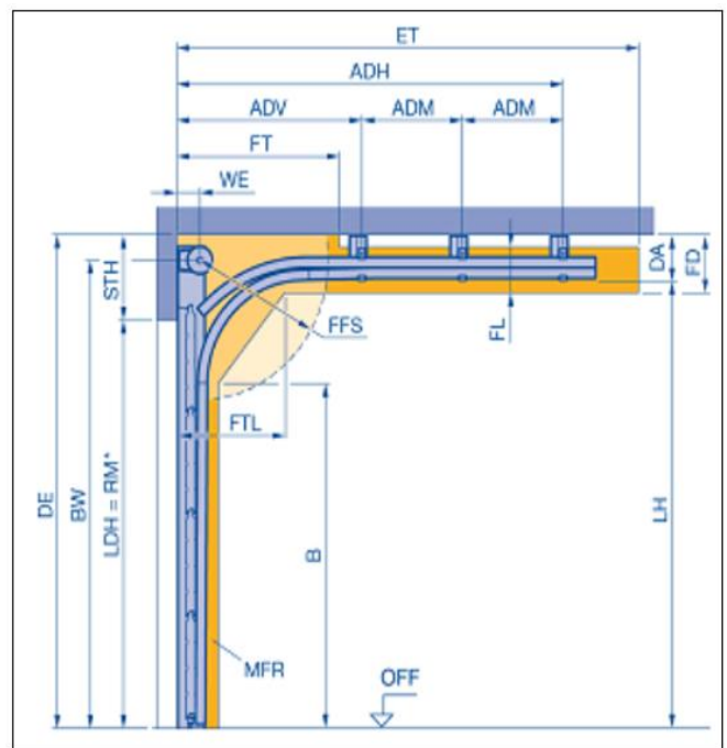
SPU F42 Industrial Sectional Garage Door I-Ribbed Micrograin in RAL7006 Beige Grey 4400mm x 8000mm
